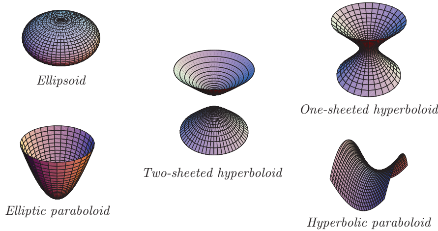
FIGURE 6. Quadrics
