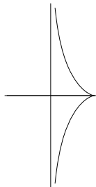
FIGURE 4. The tractrix
