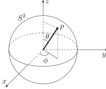
FIGURE 3. Spherical coordinates
