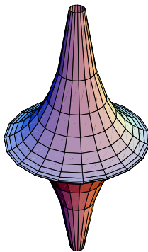
FIGURE 9. The pseudosphere
