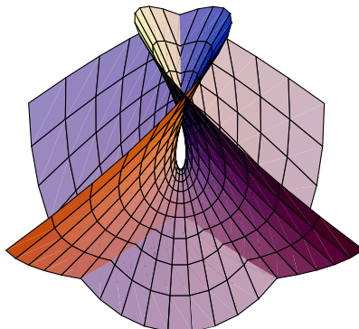
FIGURE 8. Enneper's surface
